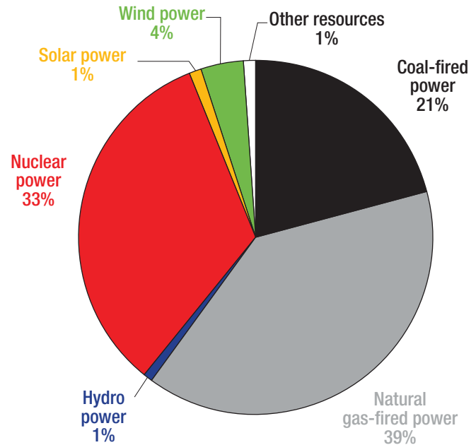
Exhibit B: Sources of Electricity Supplied for the 12 months ending June 30, 2022
